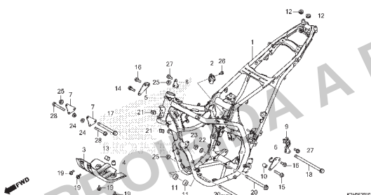
C-39 Chassi
